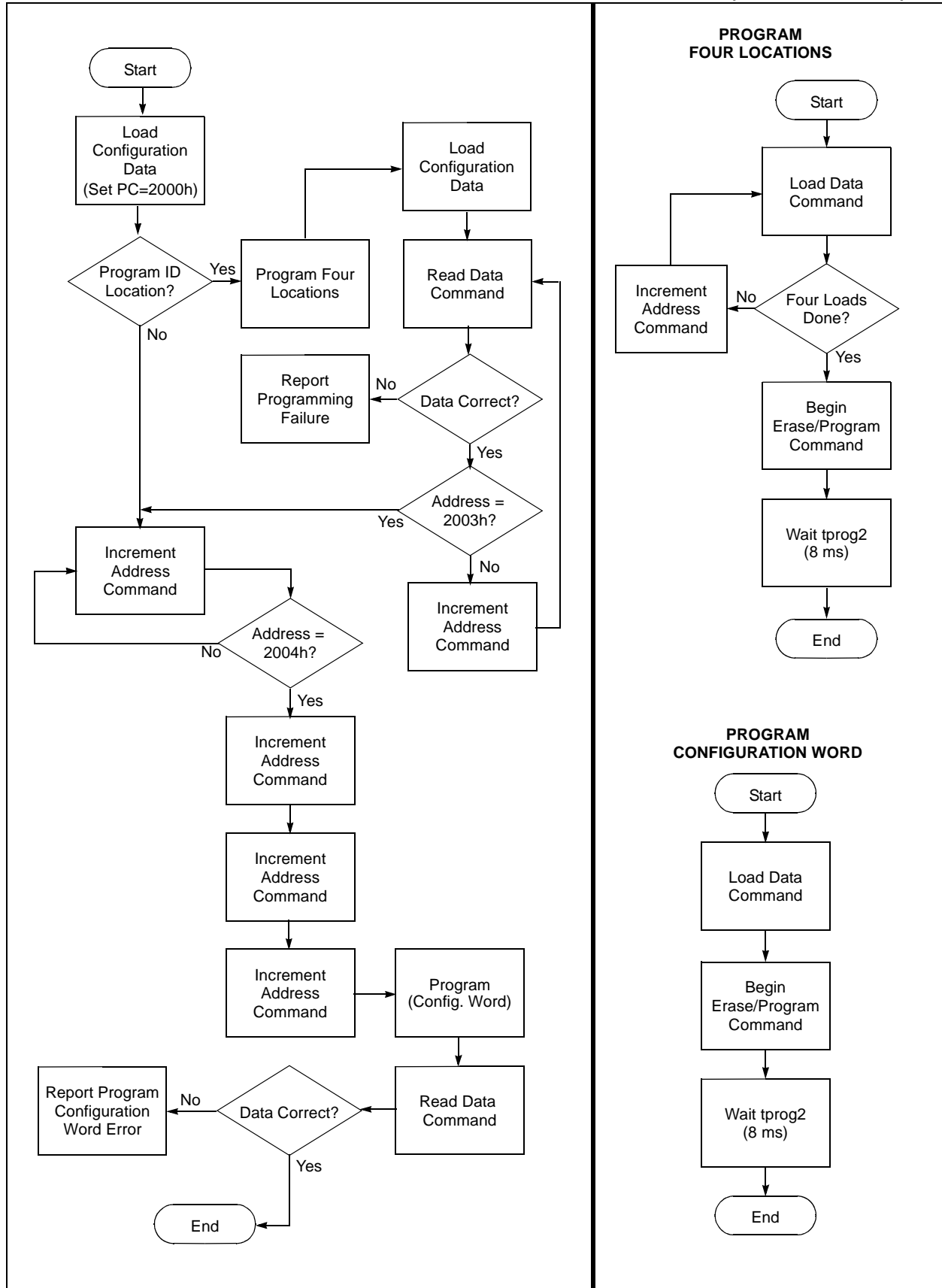
FIGURE 2-4: FLOWCHART – PIC16F87XA CONFIGURATION MEMORY (2.0V ≤ VDD < 5.5V)
