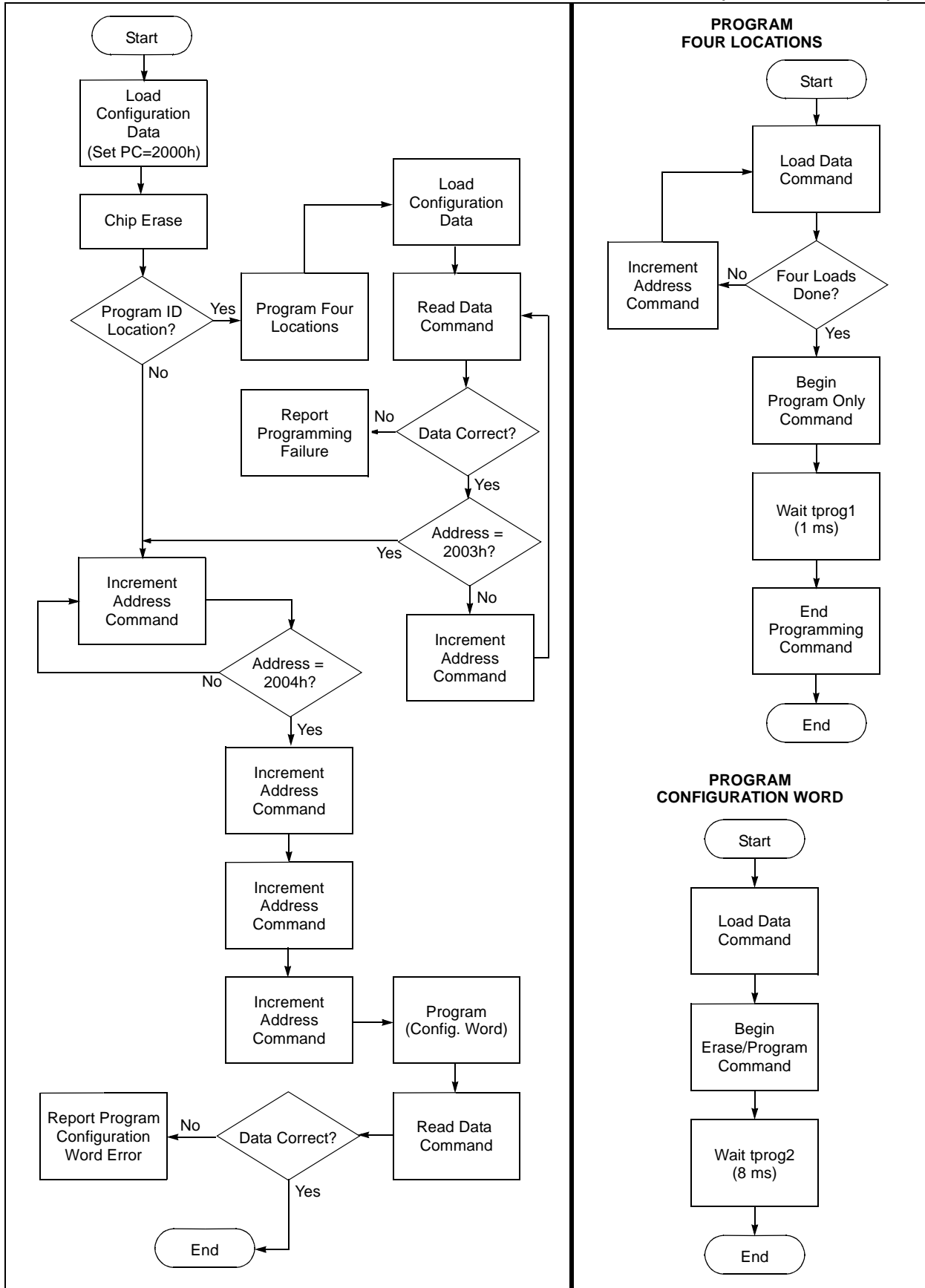
FIGURE 2-5: FLOWCHART – PIC16F87XA CONFIGURATION MEMORY (4.5V ≤ VDD ≤ 5.5V)
