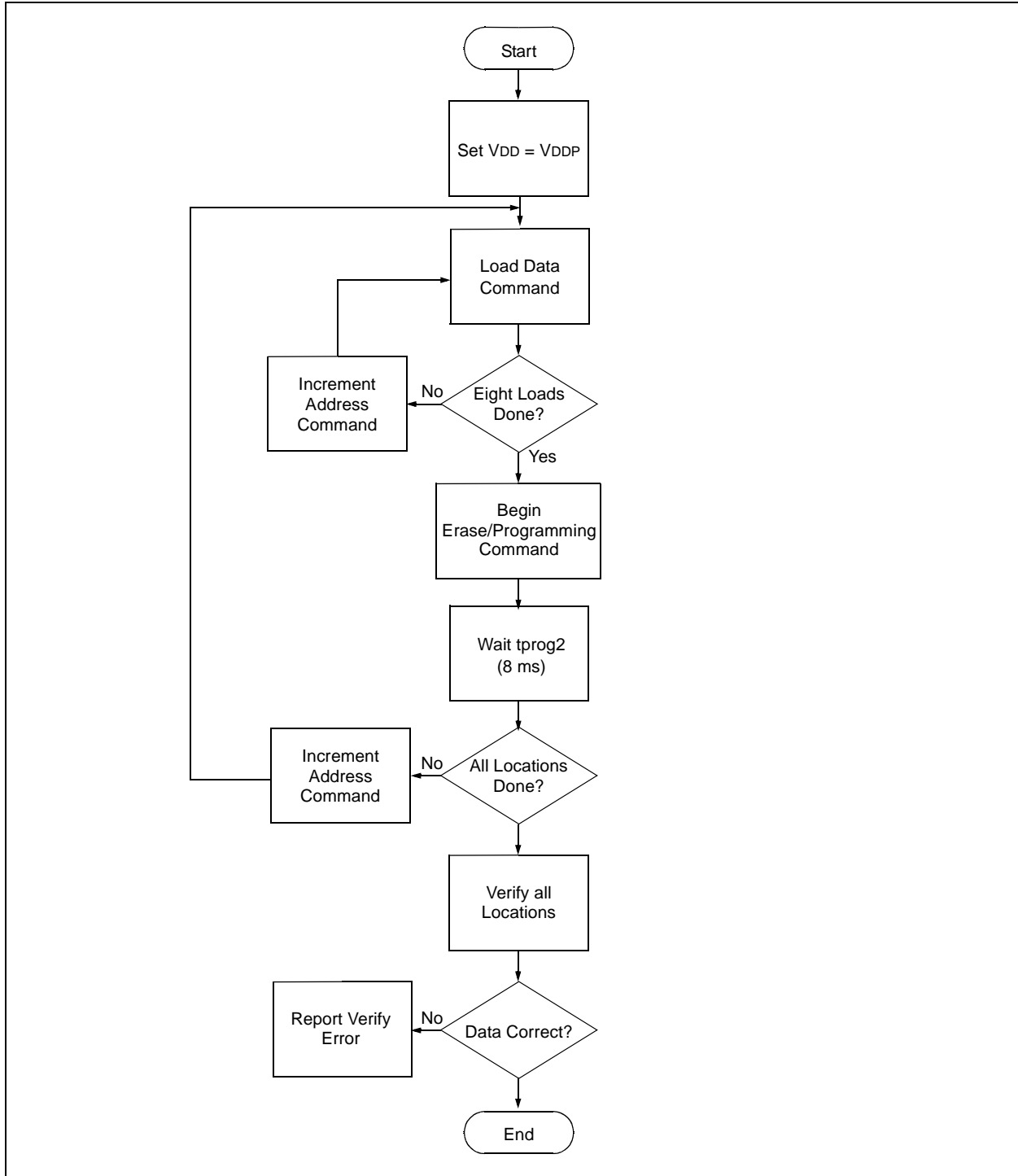
FIGURE 2-2: ALGORITHM 1 FLOWCHART – PROGRAM MEMORY (2.0V ≤ VDD < 5.5V)
