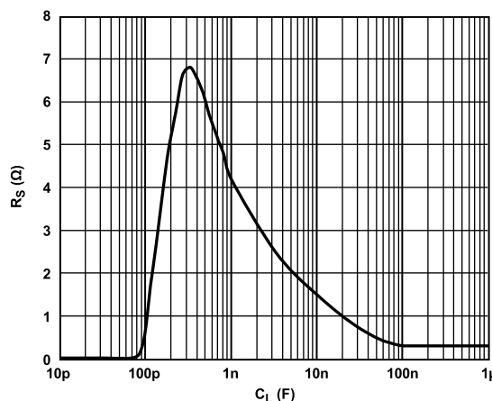
Figure 70. R_S vs. C_L for Maximum 1 dB Peaking for Circuit from Figure 69
