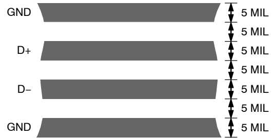
Figure 23. Typical Arrangement of Signal Tracks
