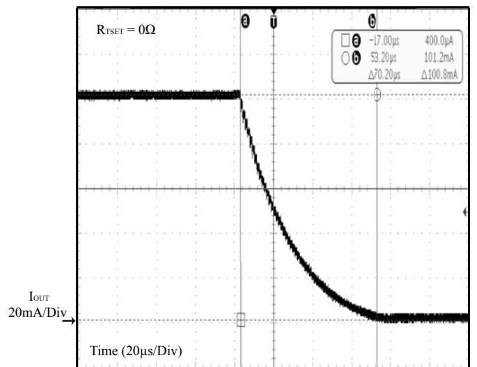
Figure 13 Instant Off
