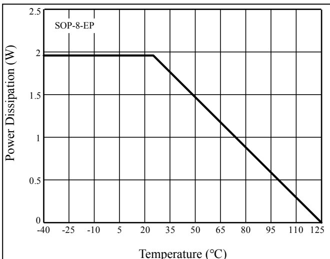
Figure 28 Dissipation Curve
