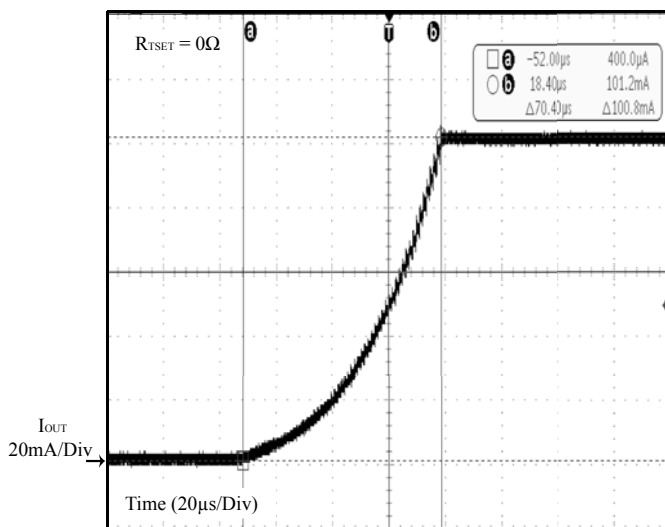
Figure 12 Instant on
