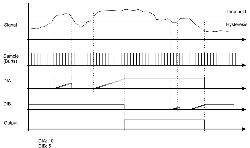
Figure 2-2 Detect Integrators Operation (Positive mode, Section 2.8.2)
