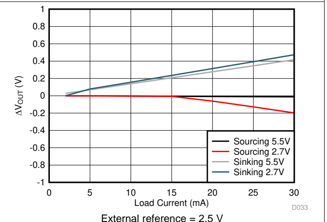
Figure 32. Headroom and Footroom vs Load Current
