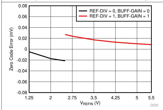
Figure 23. Zero Code Error vs Reference Voltage
