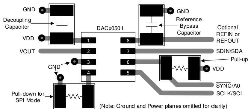
Figure 73. Layout Example
