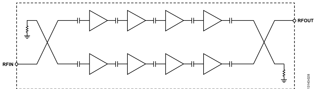
Figure 34. HMC1144 Architecture
