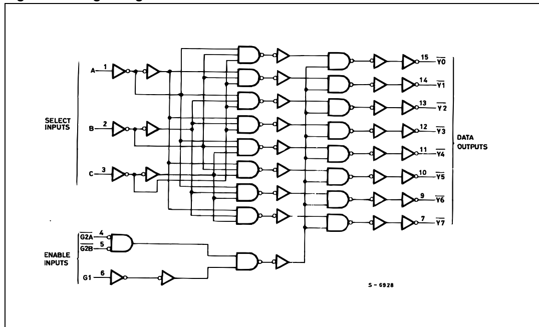
Figure 4. Logic diagram
