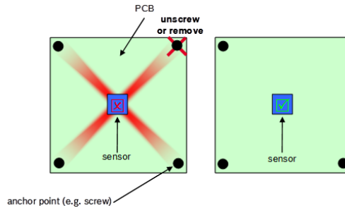
Figure 3: redundant PCB anchor points
