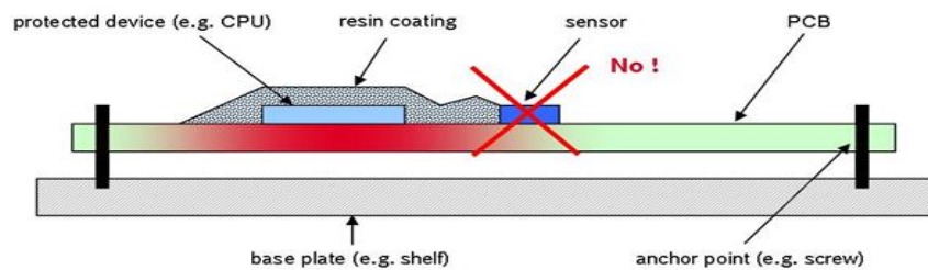
Figure 7: Resin coatings
