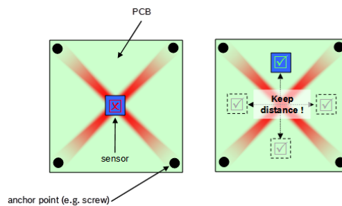
Figure 4: Mechanical stress maximum on the PCB
