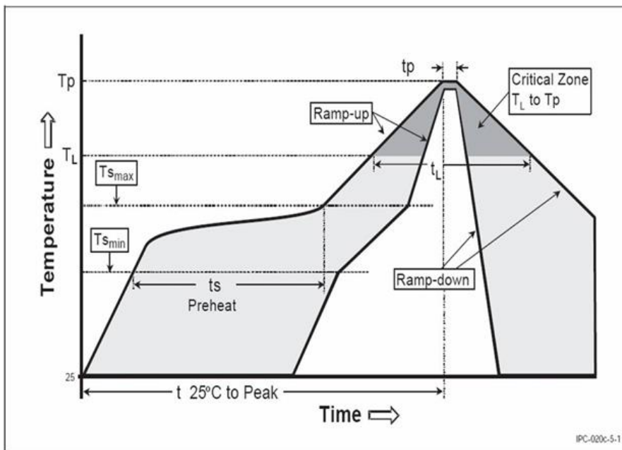
Figure 11: Multiple reflow soldering cycle – Temperature Vs Time curve
