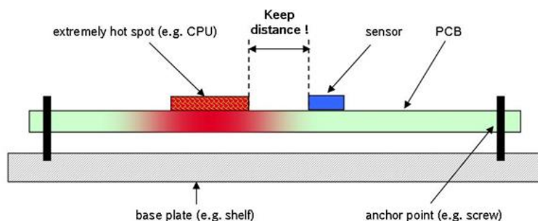
Figure 2: Thermal hot-spots on the PCB
