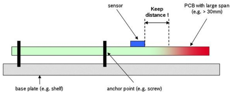
Figure 6: Vibrating PCB
