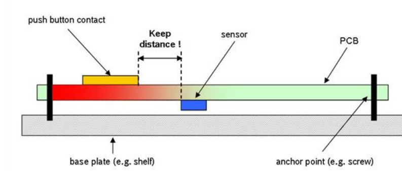
Figure 1: Push-button contacts
