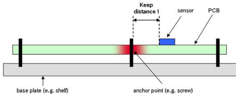
Figure 5: Distance to PCB anchor points
