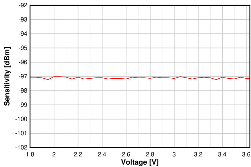
Figure 8-14. Sensitivity vs. Supply Voltage (VDDS) (BLE 1 Mbps, 2.44 GHz, DCDC Off)
