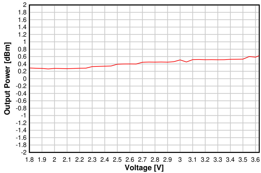
Figure 8-18. Output Power vs. Supply Voltage (VDDS) (BLE 1 Mbps, 2.44 GHz)
