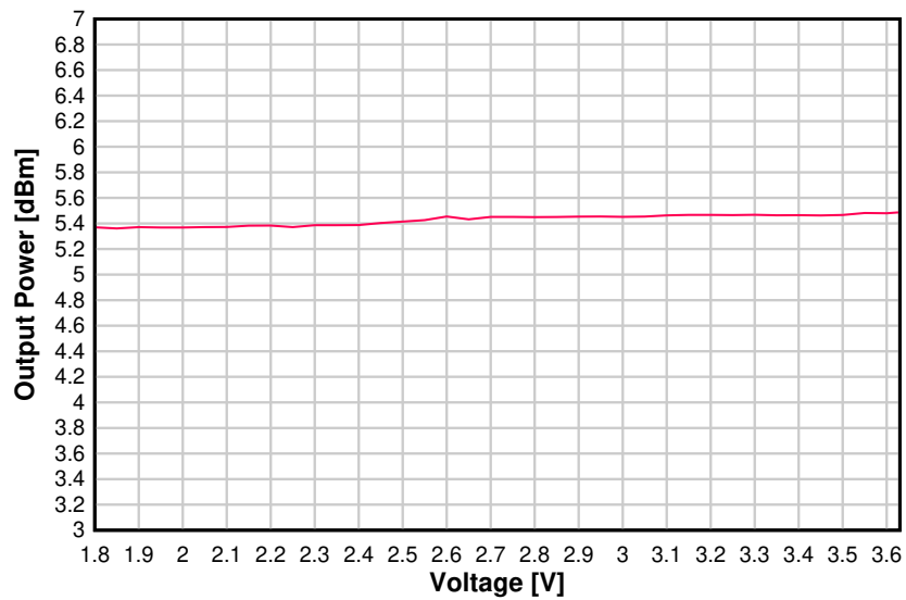
Figure 8-19. Output Power vs. Supply Voltage (VDDS) (BLE 1 Mbps, 2.44 GHz, +5 dBm)
