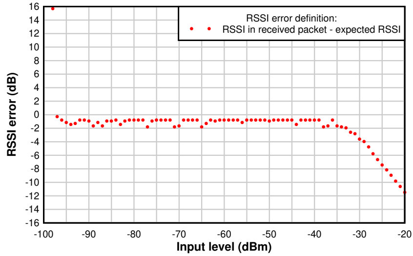
Figure 8-15. RSSI Error vs. Input Level (dBm) (BLE 1 Mbps)
