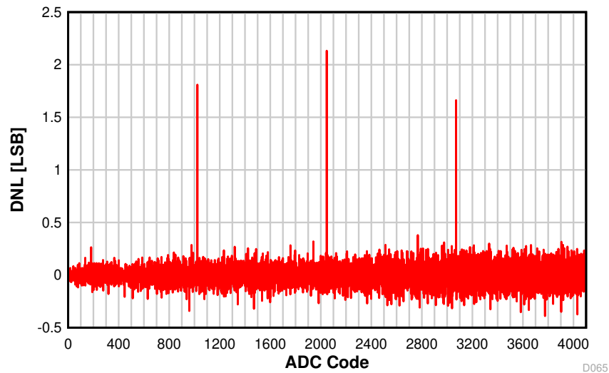
Figure 8-25. DNL vs. ADC Code
