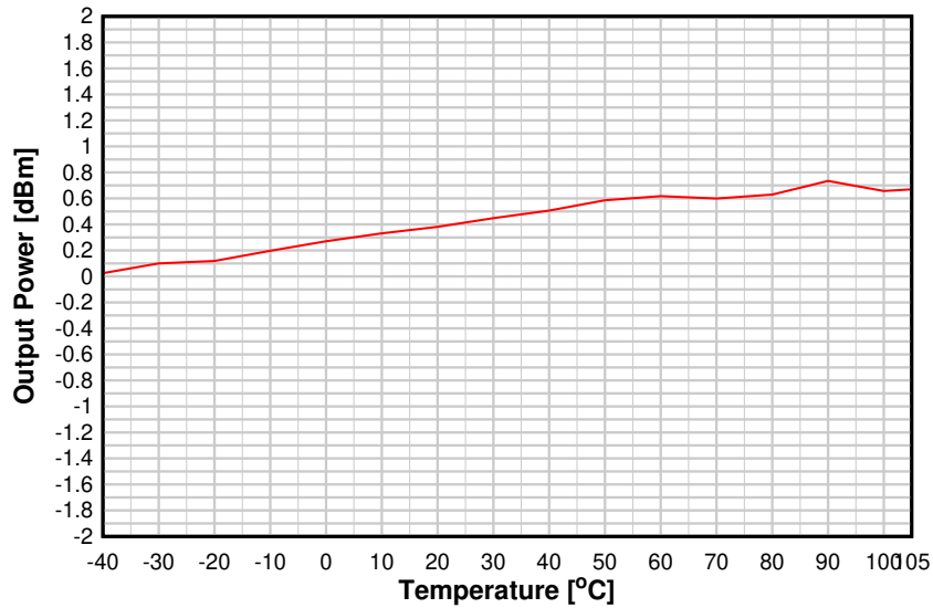
Figure 8-16. Output Power vs. Temperature (BLE 1 Mbps, 2.44 GHz)
