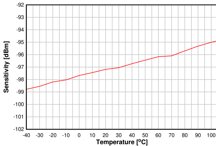
Figure 8-12. Sensitivity vs. Temperature (BLE 1 Mbps, 2.44 GHz)
