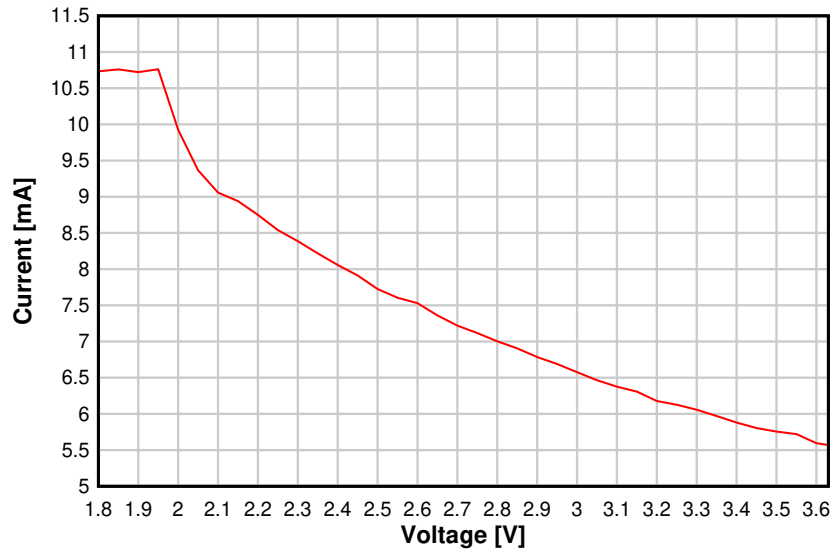
Figure 8-8. RX Current vs. Supply Voltage (VDD5) (BLE 1 Mbps, 2.44 GHz)
