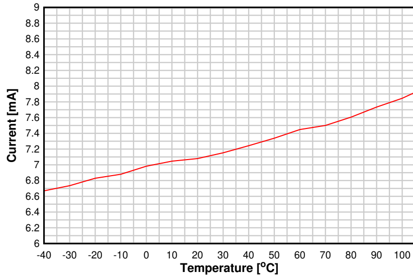
Figure 8-9. TX Current vs. Temperature (BLE 1 Mbps, 2.44 GHz)
