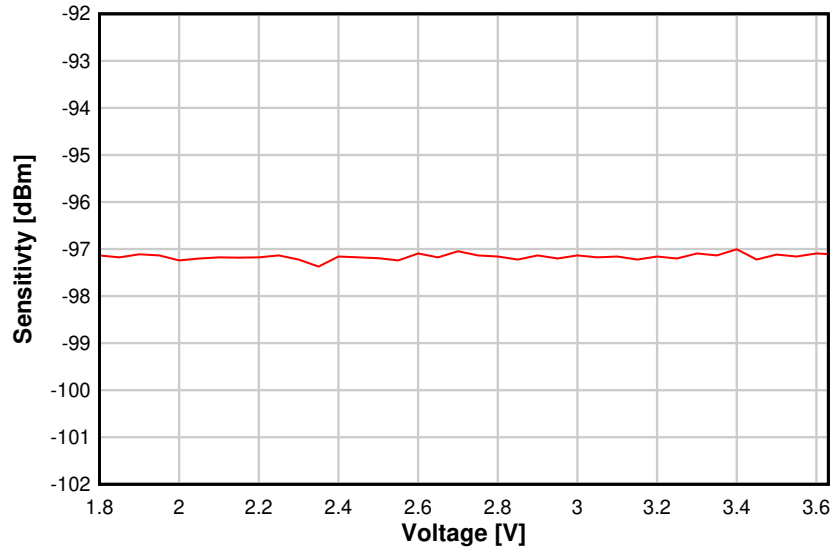
Figure 8-13. Sensitivity vs. Supply Voltage (VDDS) (BLE 1 Mbps, 2.44 GHz)
