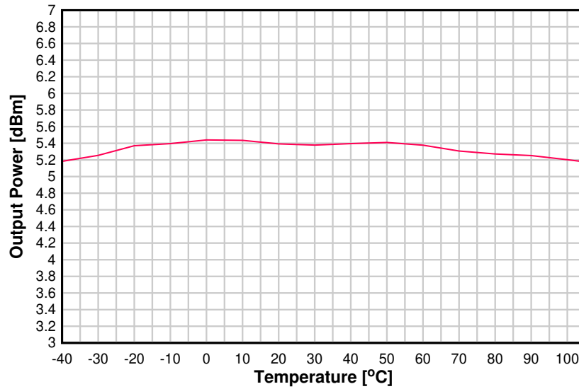
Figure 8-17. Output Power vs. Temperature (BLE 1 Mbps, 2.44 GHz, +5 dBm)
