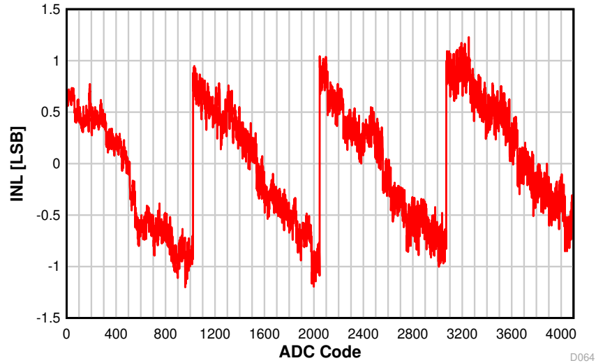
Figure 8-24. INL vs. ADC Code
