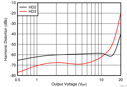
f = 10 MHz, A_V = 10\text{ V/V} Figure 6-20. Harmonic Distortion vs V_O
