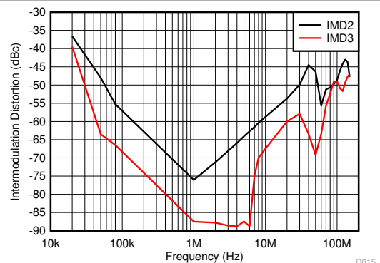
\pm 12.2\text{ kHz} tone spacing, V_O = 2\text{ V}_{PP} per tone Figure 6-23. Intermodulation Distortion vs Frequency
