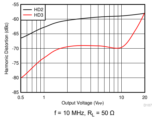
Figure 6-46. Harmonic Distortion vs V_O
