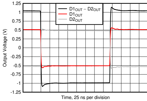
Figure 6-49. Small-Signal Pulse Response
