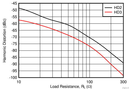
f = 10 MHz, V_O = 2\text{ V}_{PP} , A_V = 10\text{ V/V} Figure 6-22. Harmonic Distortion vs R_L
