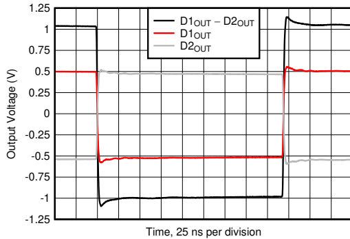
Figure 6-25. Small-Signal Pulse Response
