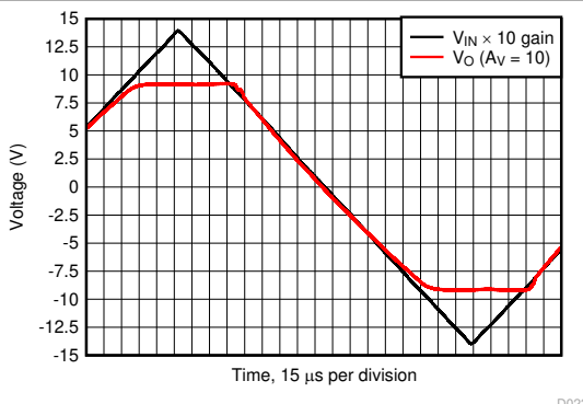
V_{IN} = 2.8\text{-V}_{PP} triangular waveform Figure 6-24. Overdrive Recovery
