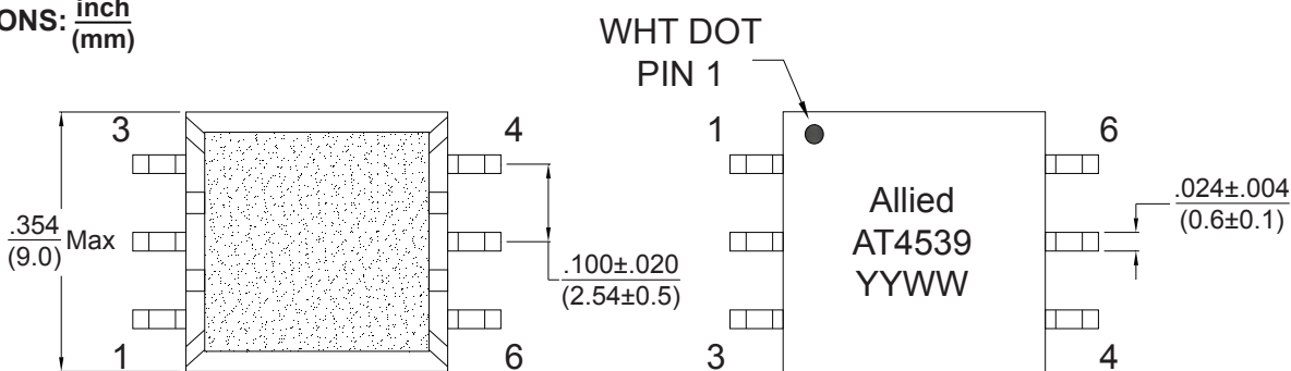
BOTTOM VIEW
